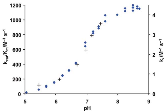
Fig. 4 Plot of k_{cat}/K_m for the hydrolysis of N -suc(L-Ala) 3 - p -nitroanilide by PPelastase (◆) and k_i for N -benzoyl- \beta -sultam (3) with PPelastase (+) against pH. 30 °C, I = 1.0 M (KCl), 6 % MeCN v/v and 1.5% MeOH v/v.
